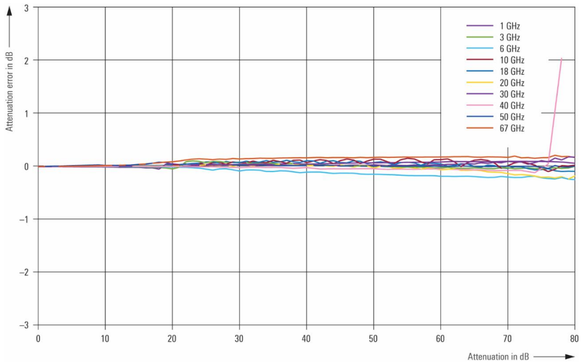
Measured level linearity of high dynamic uninterrupted level sweep with the R&amp;S®SMAB-K724 option
