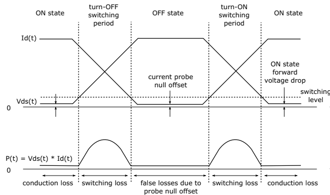
Figure 6 Loss Occurrence in the Power Device
