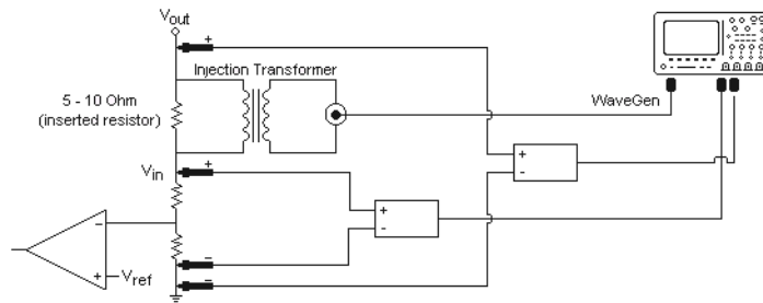
Figure 15 Typical Configuration for Control Loop Response Analysis
