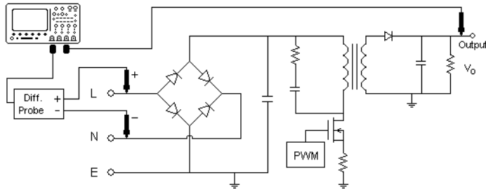
Figure 11 Typical Configuration for Turn On/Off Analysis Tests
