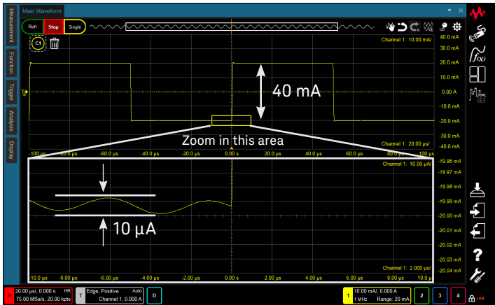
Figure 3. Wide dynamic range measurement example: 40 mA and 10 μA current waveform measurements at the same time.
