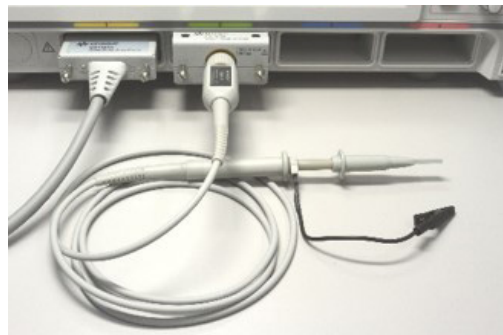
Figure 7. The CX3300 series can also measure and view voltage waveforms using a passive probe, so that you can view the dynamic power waveforms as well as current waveforms.
