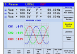
Interharmonics Waveform
