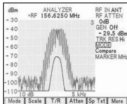
The IFR-1900 CSA gives you full featured service monitor functions
