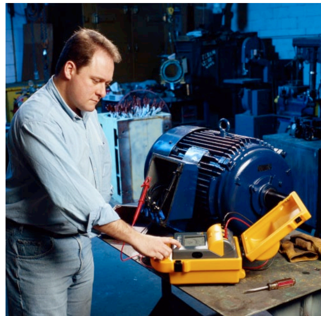
MegOhmMeter insulation resistance tester
